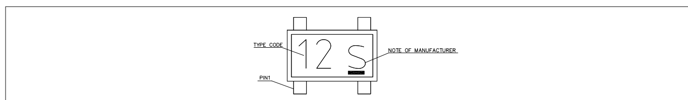
Figure 24 Marking layout example
