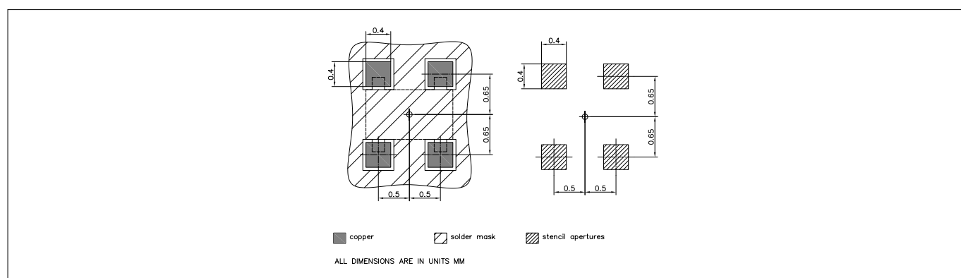
Figure 23 Foot print
