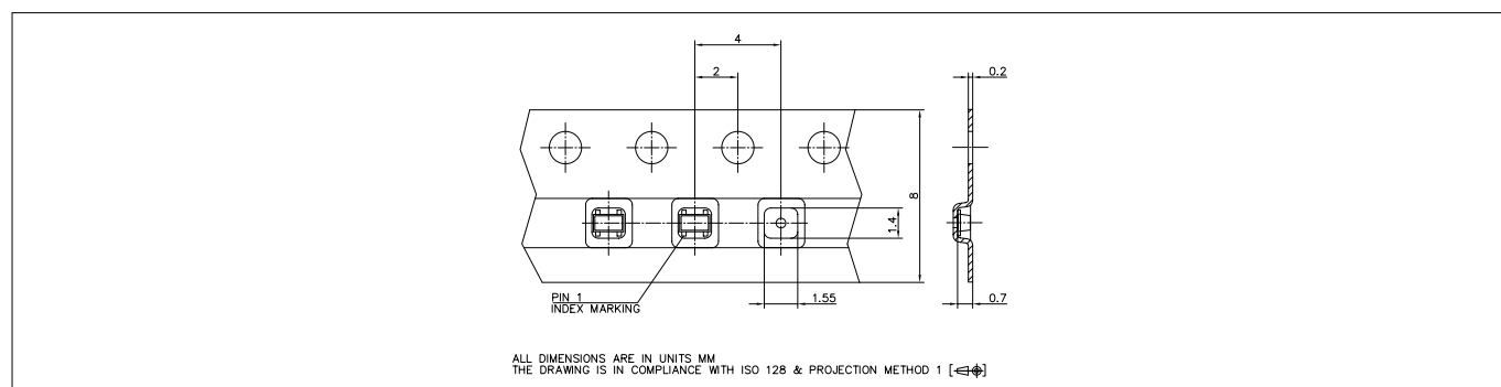
Figure 25 Tape dimensions
